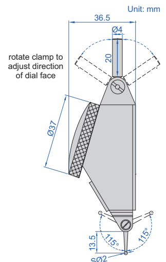
clamp (included)
