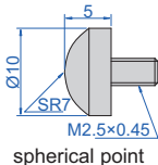
spherical point
